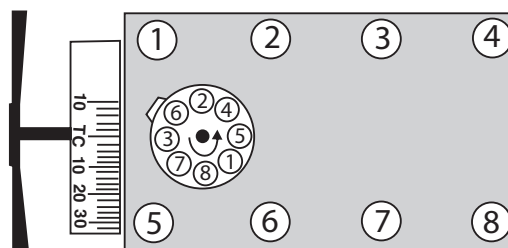
Figura 2 - Ford V8 de 289 a 302 c.i.d.
